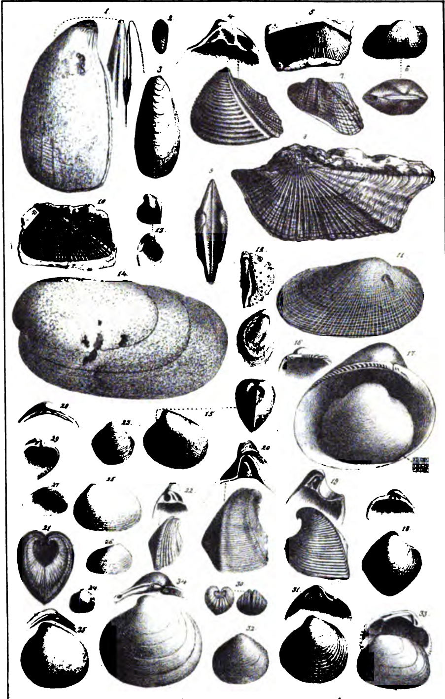
Buenstall, sura
